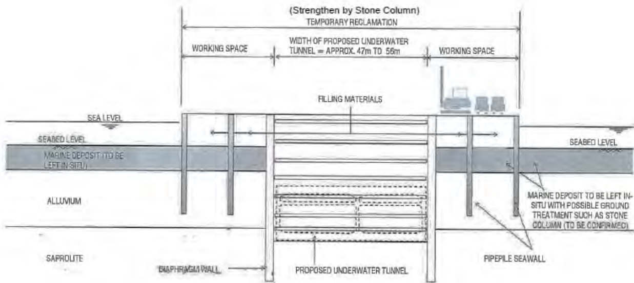
Figure 1 – Original Scheme for Temporary Reclamation stated in the CKR EIA Report
