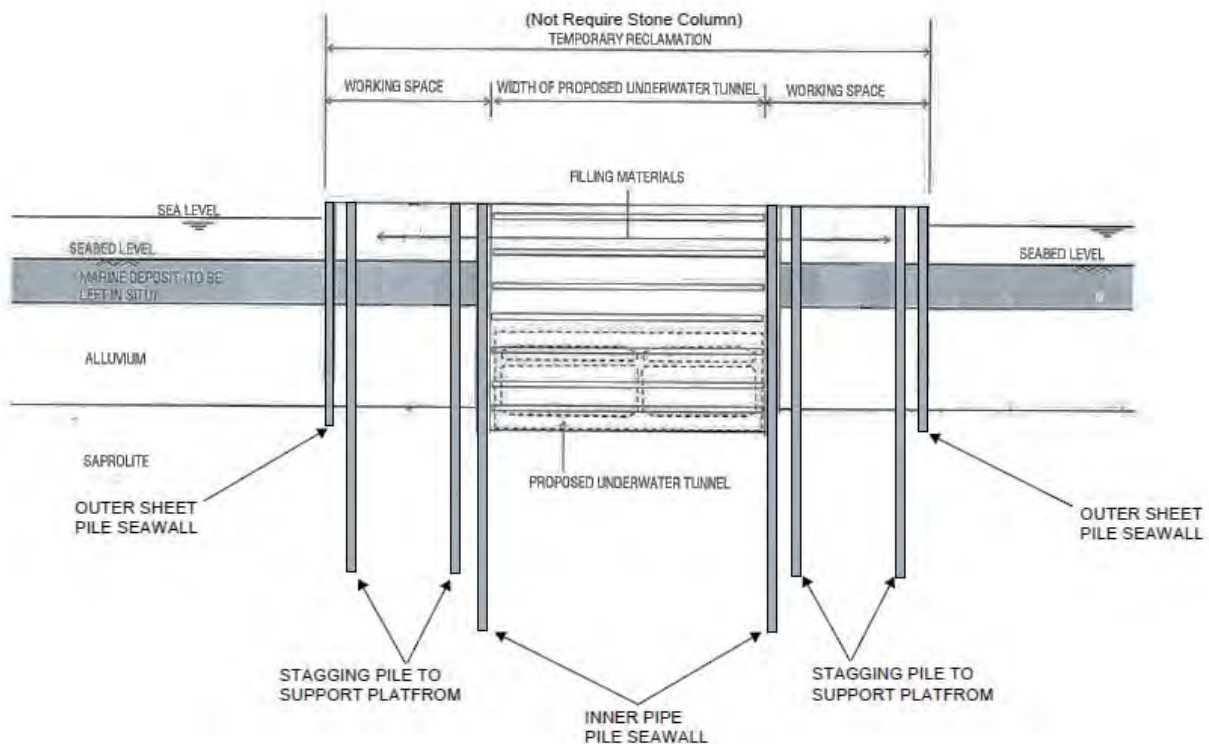
Figure 2 – Proposed Scheme for Temporary Reclamation
